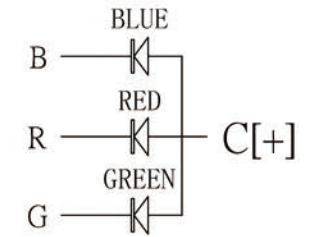
LED CIRCUIT
